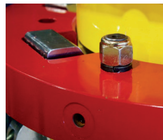
The mechanical locking ring secures the cams in place even during a loss of hydraulic power.
